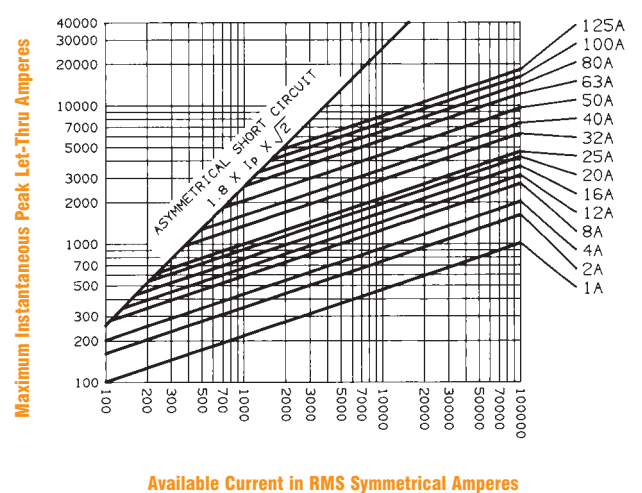
Peak Let-Thru Current Data – 1-125 Amperes
